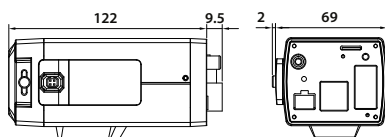
[LNB5110_Side]
